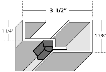
16 GA. STEEL FRAME DUAL CONTACT WEATHER STRIP
