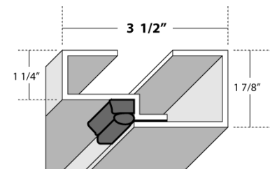
16 GA. STEEL FRAME DUAL CONTACT WEATHER STRIP
