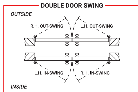
Must specify active door panel when ordering double doors
