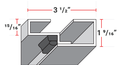
DUAL CONTACT WEATHER STRIP
