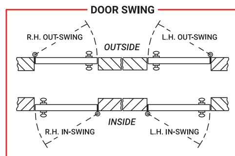
Must specify door swing when ordering doors with windows
