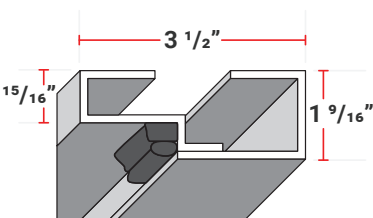
DUAL CONTACT WEATHER STRIP
